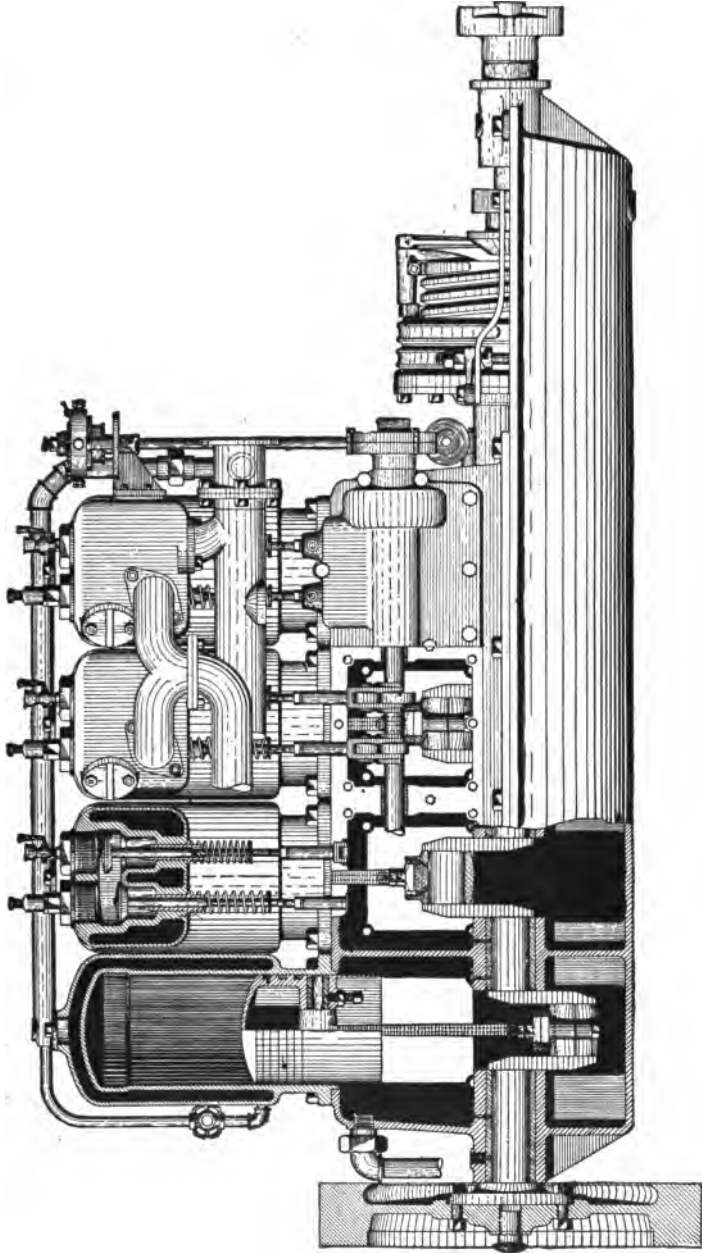
FIG. 80.—Jaeger Engine.
